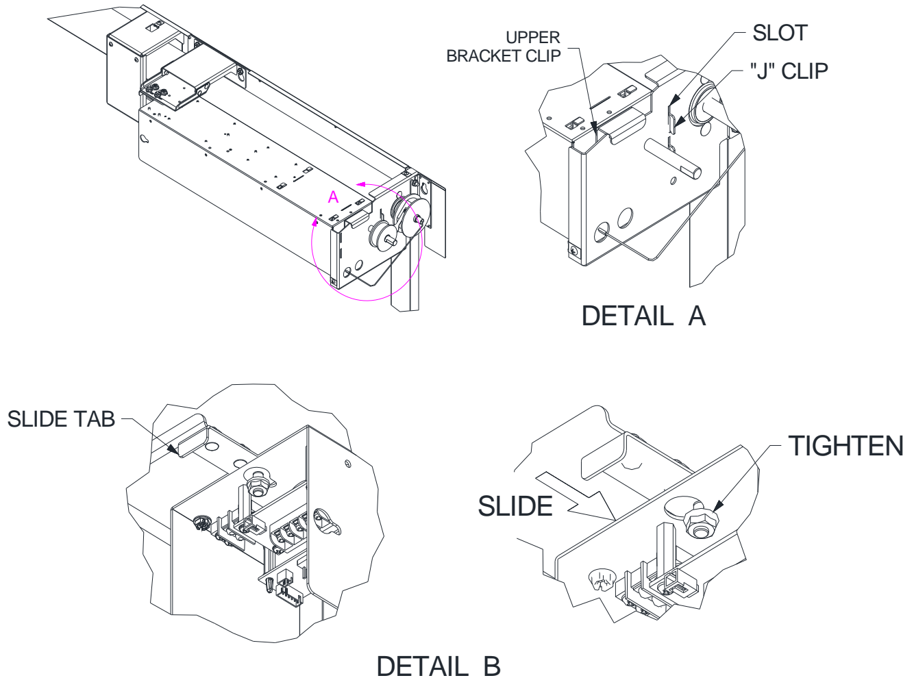
Figure 5.12a – Installing Standard Control Box
