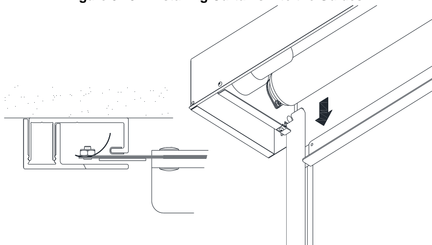
Figure 5.19 – Installing Curtains into the Guides
