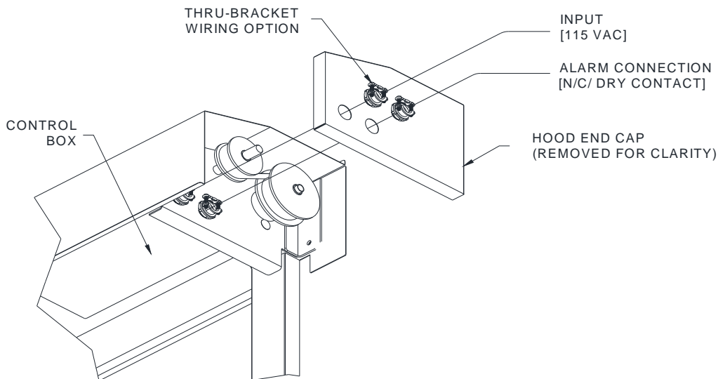
Figure 5.23 – Input Wiring
