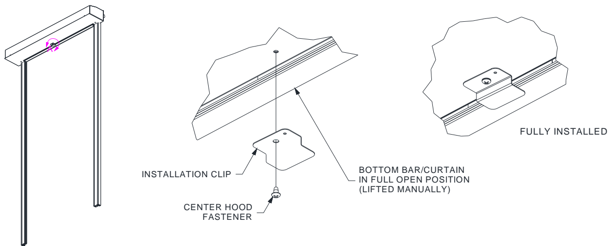
Figure 5.26 – Holding Door in Open Position without Power
