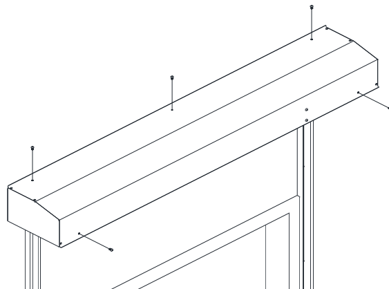
Figure 5.14 – Installing Hood
