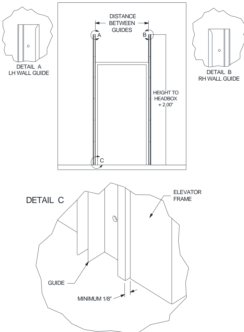
Figure 5.1 - Wall Guides
