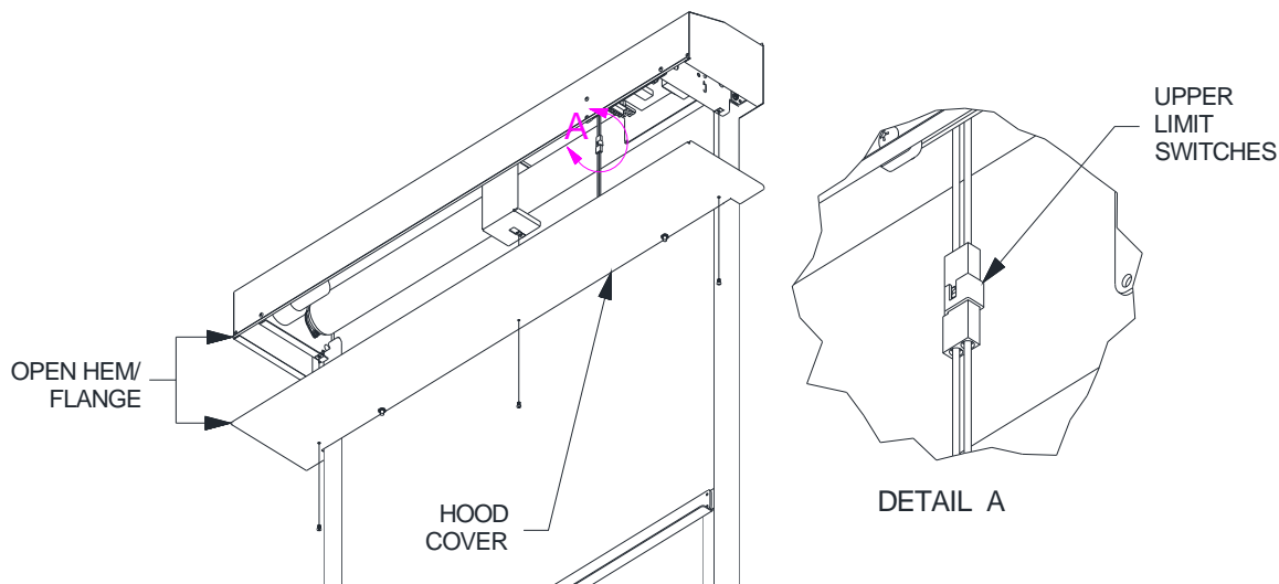
Figure 5.25 – Installing Hood Cover
