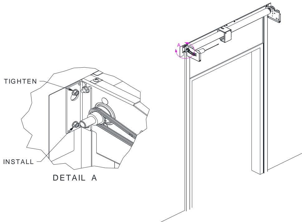
Figure 5.9 – Installing Headbox
