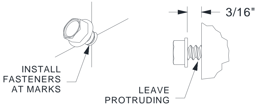
Figure 5.5 – Installing Wall Fasteners
