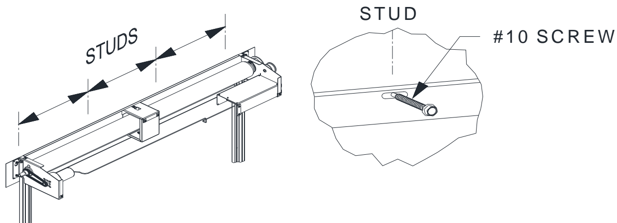
Figure 5.10 – Mounting Plate Wall Fasteners
