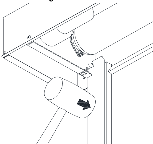
Figure 5.17 – Strike Method
