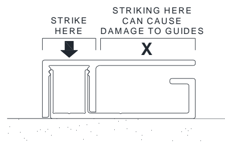
Figure 5.18 – Snap Direction
