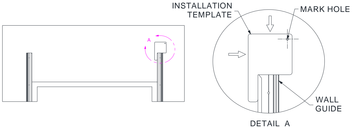
Figure 5.3 – Marking Wall Fastener Locations
