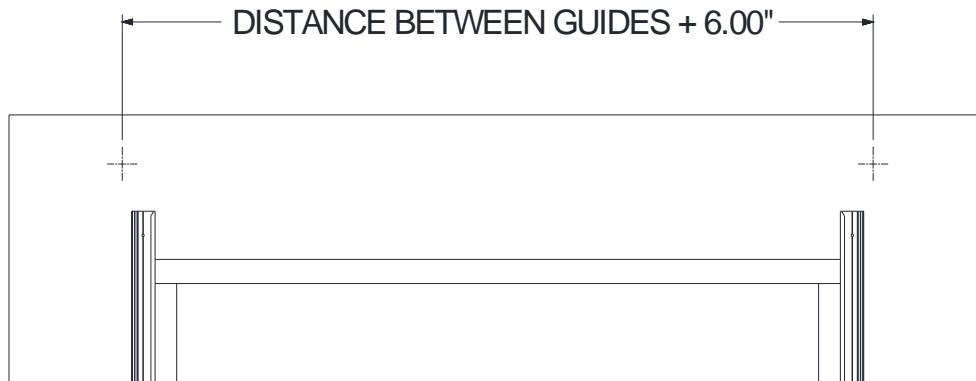
Figure 5.4 – Measuring Fastener Location Distance
